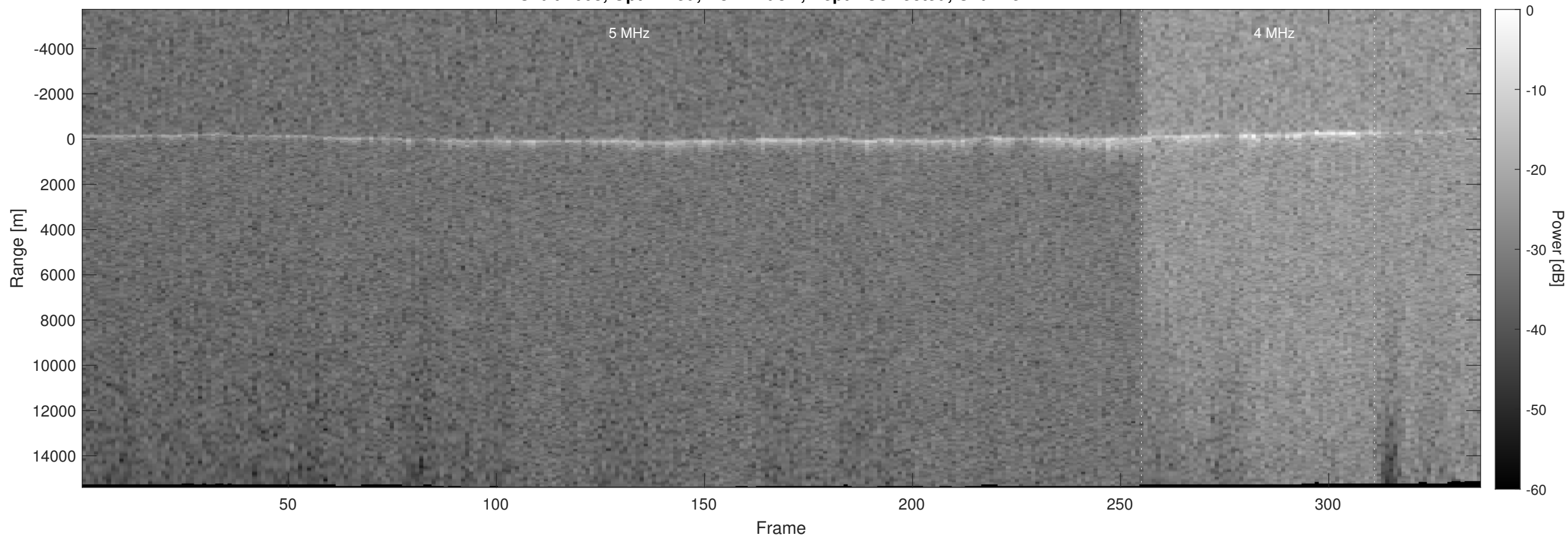
Orbit 2008, Optimized, No Window, Depth-Corrected, Channel 2
