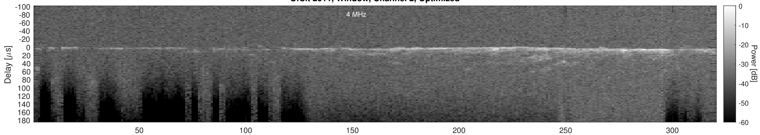
Orbit 2011, Cluttergram
