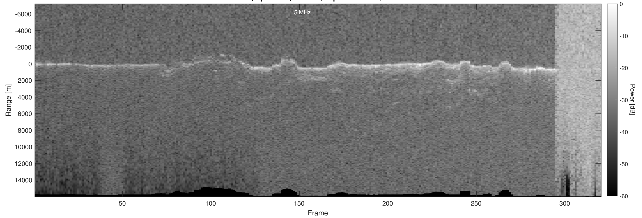
Orbit 2011, Optimized, Window, Depth-Corrected, Channel 2
