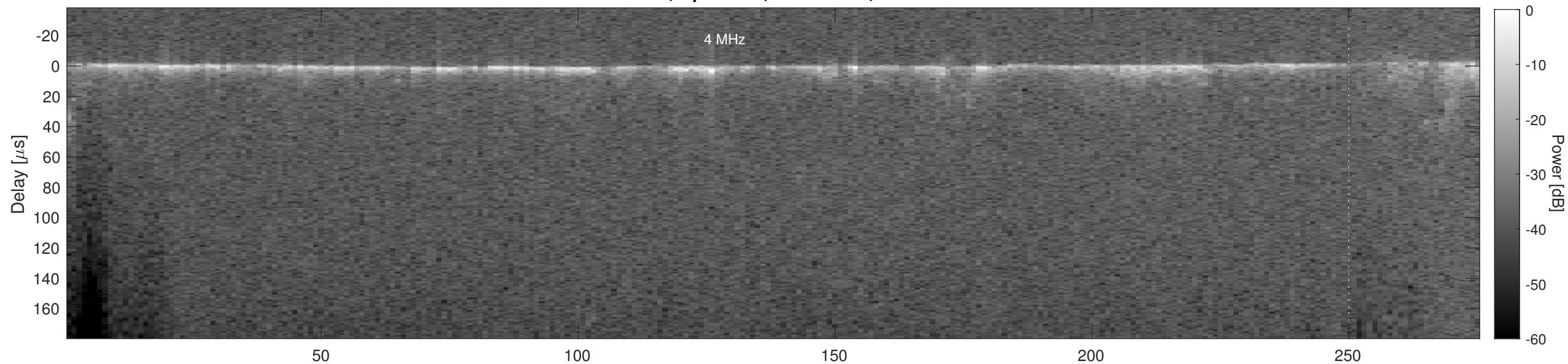
Orbit 2019, Cluttergram
