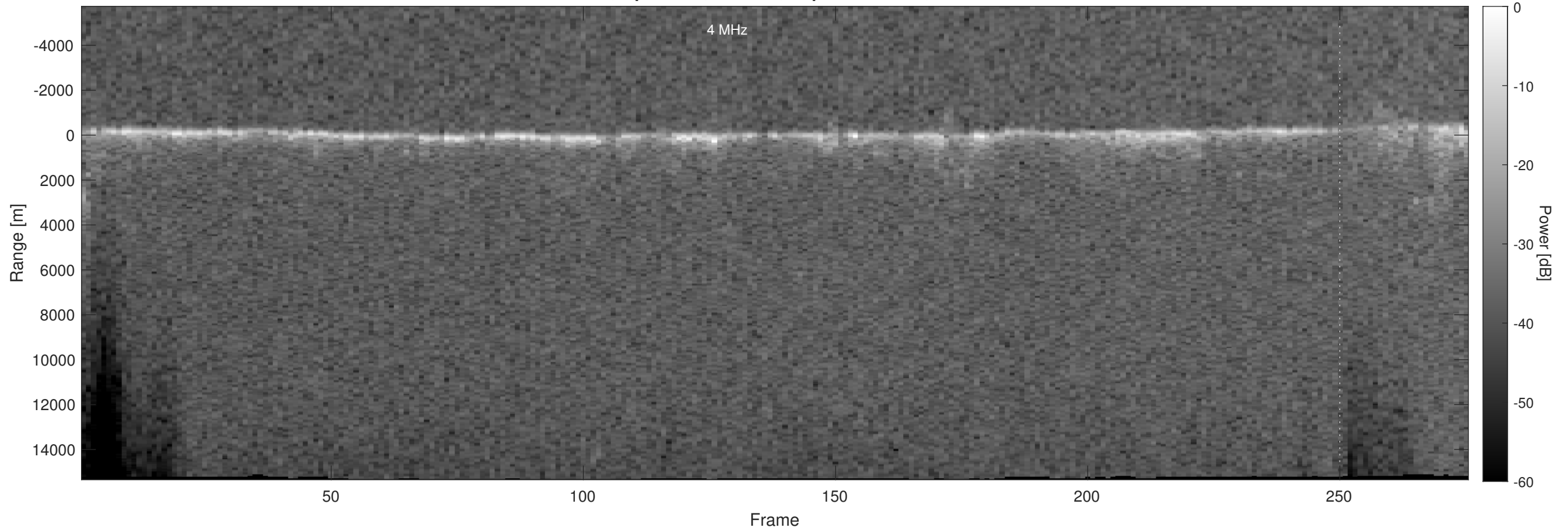
Orbit 2019, Optimized, Window, Depth-Corrected, Channel 2
