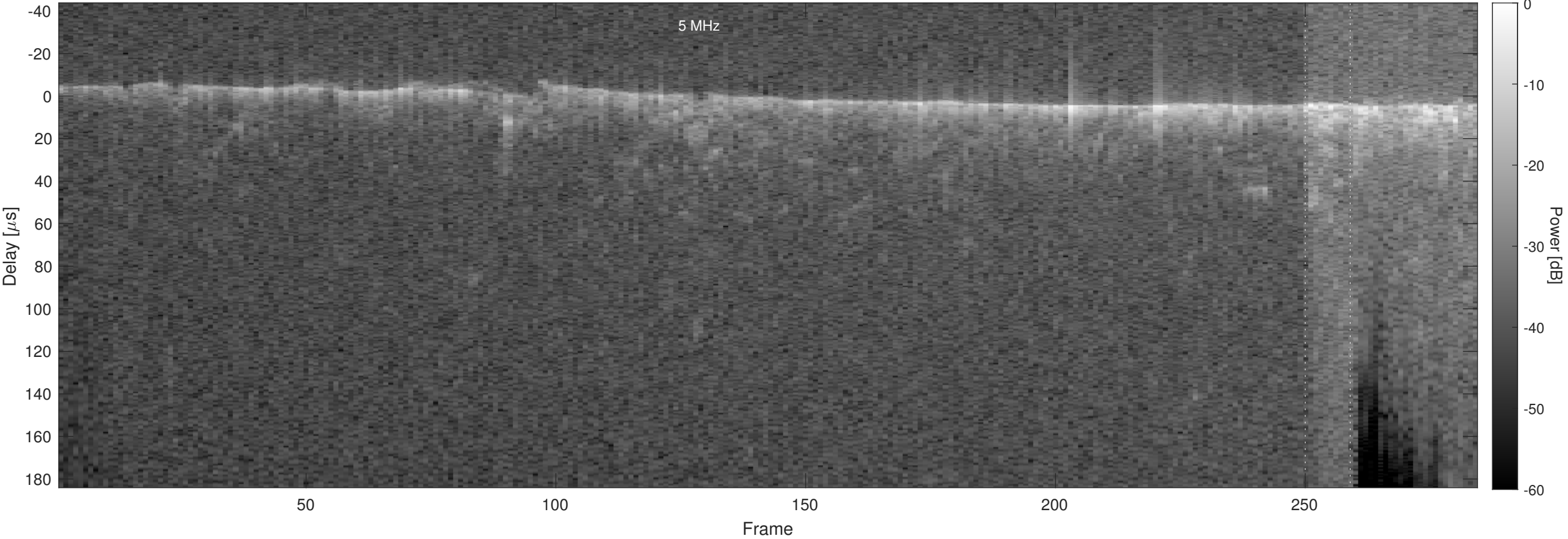
Orbit 2020, Optimized, No Window, Channel 2
