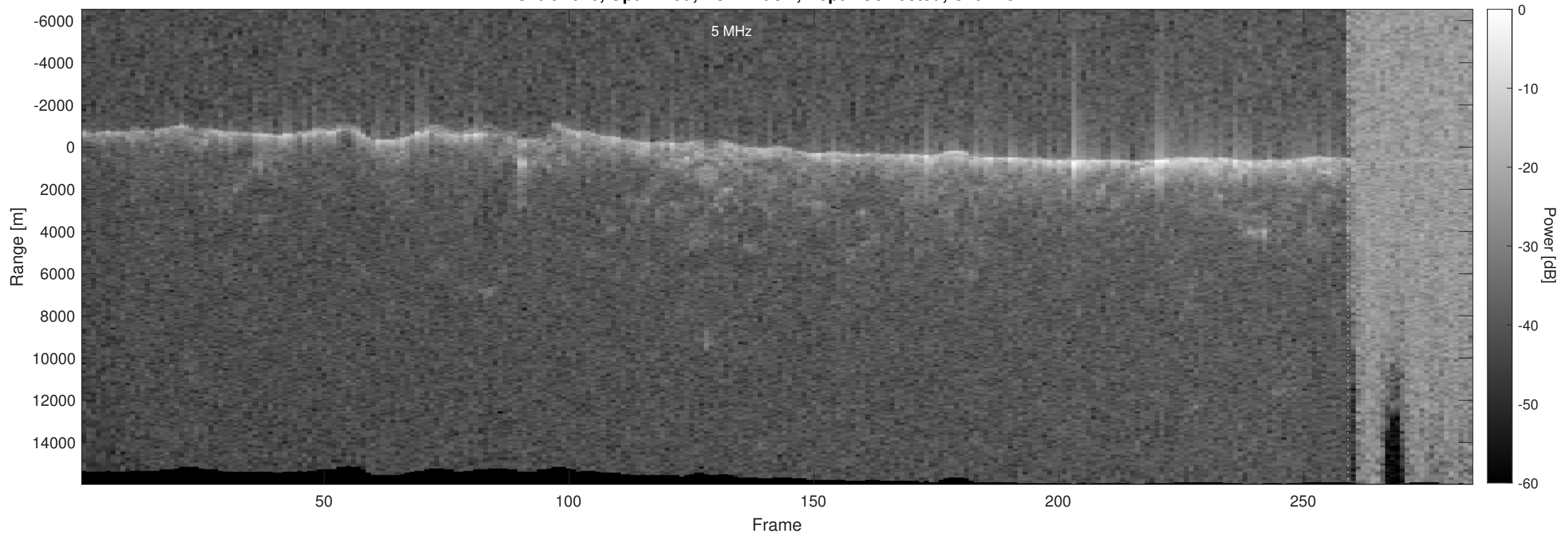
Orbit 2020, Optimized, No Window, Depth-Corrected, Channel 2
