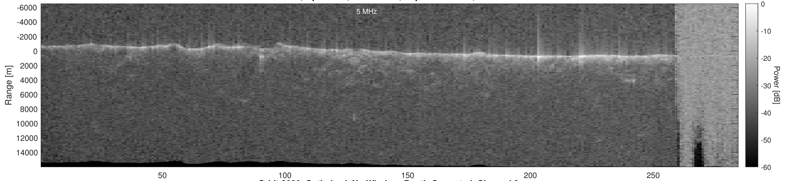
Orbit 2020, Optimized, No Window, Depth-Corrected, Channel 2
