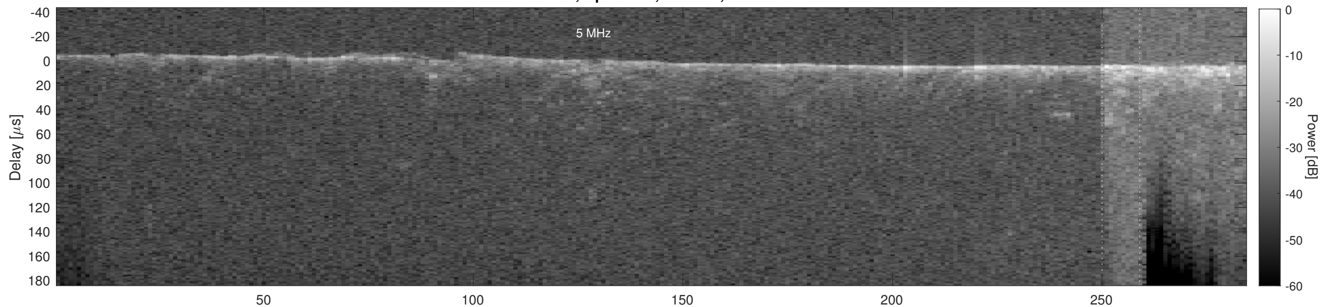
Orbit 2020, Cluttergram
