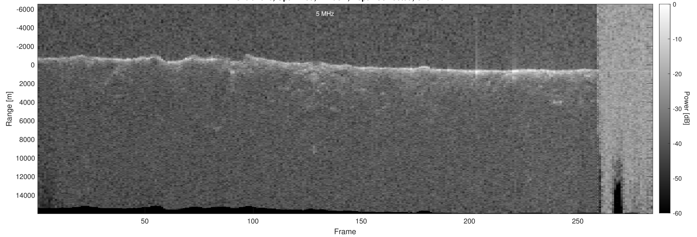
Orbit 2020, Optimized, Window, Depth-Corrected, Channel 2
