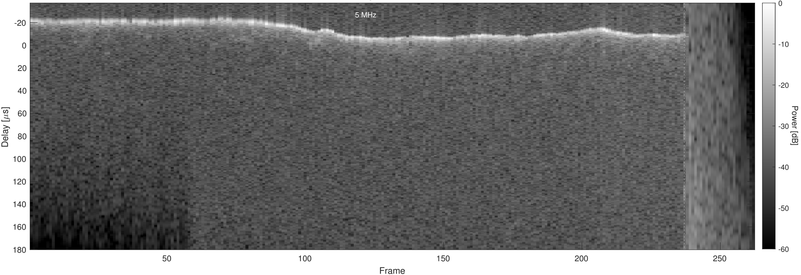
Orbit 2024, Chapman, Window, Channel 2
