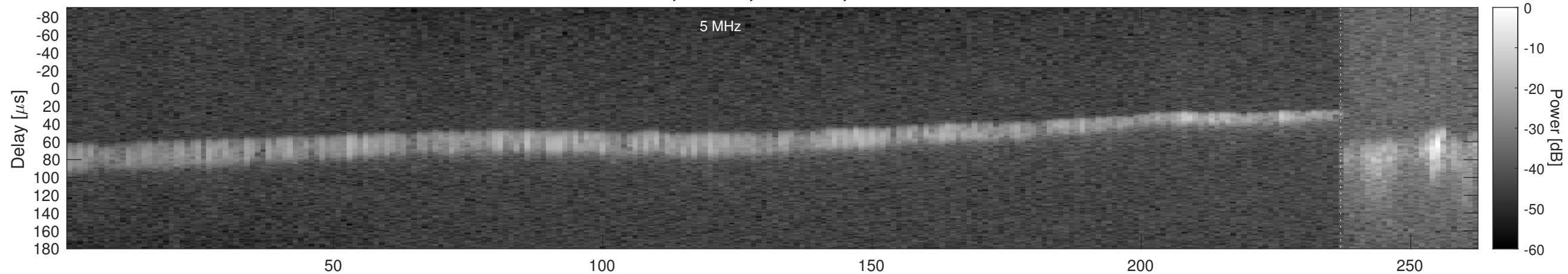
Orbit 2024, Window, Channel 2, Chapman
