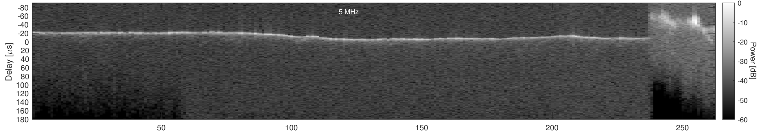
Orbit 2024, Window, Channel 2, Optimized
