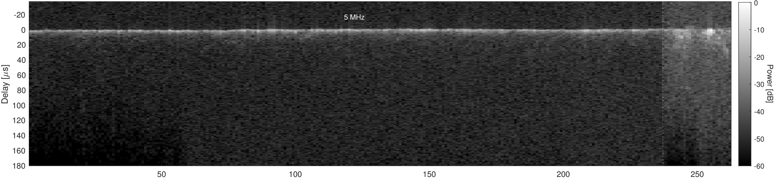
Orbit 2024, Cluttergram
