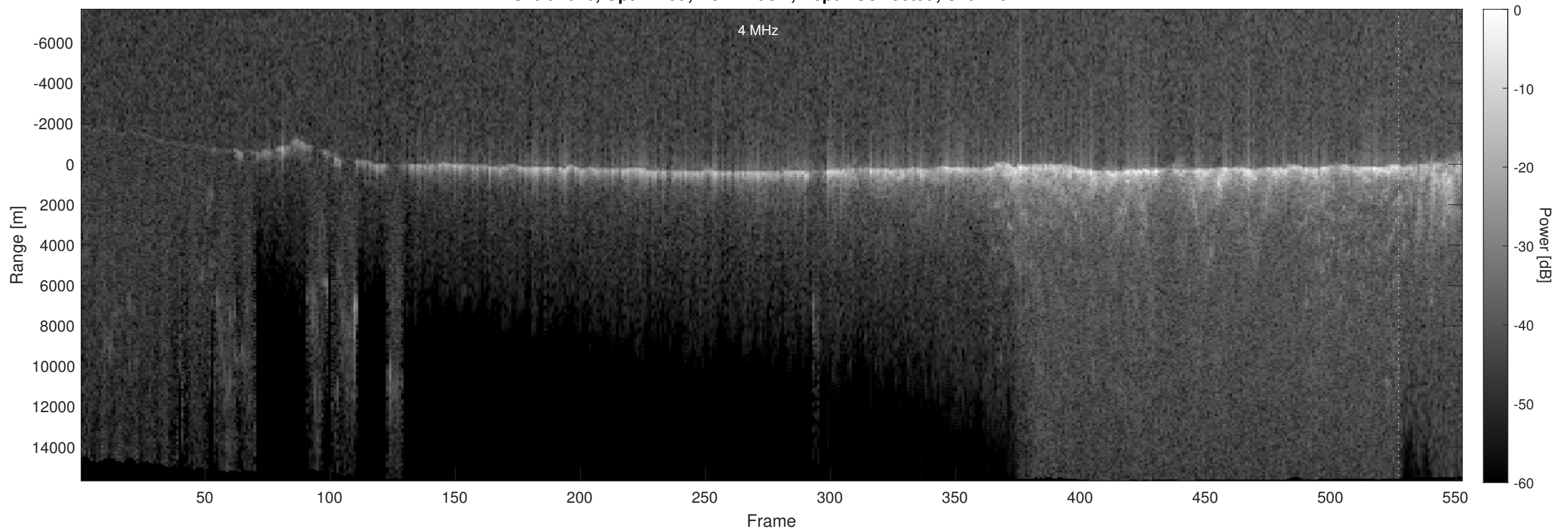
Orbit 2026, Optimized, No Window, Depth-Corrected, Channel 2
