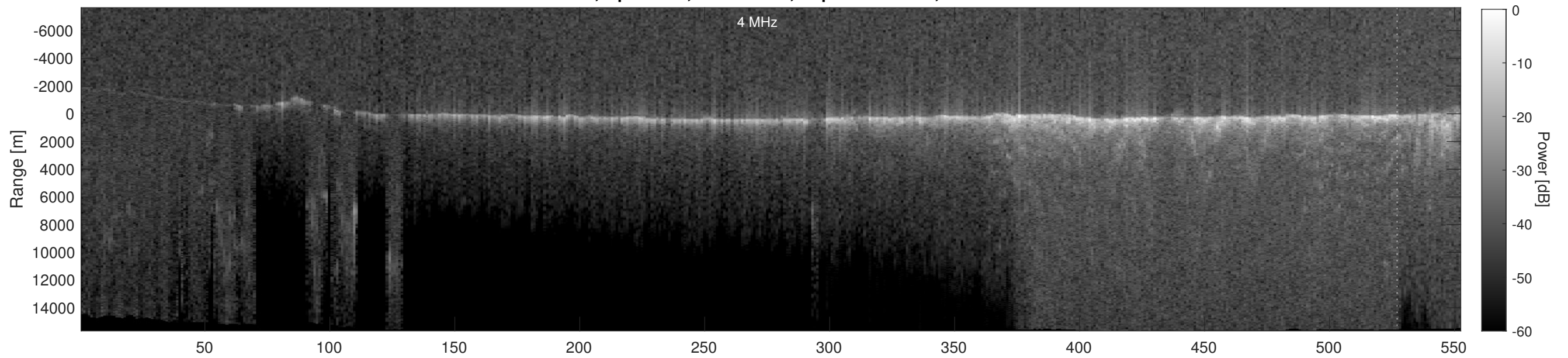
Orbit 2026, Depth-Corrected Cluttergram
