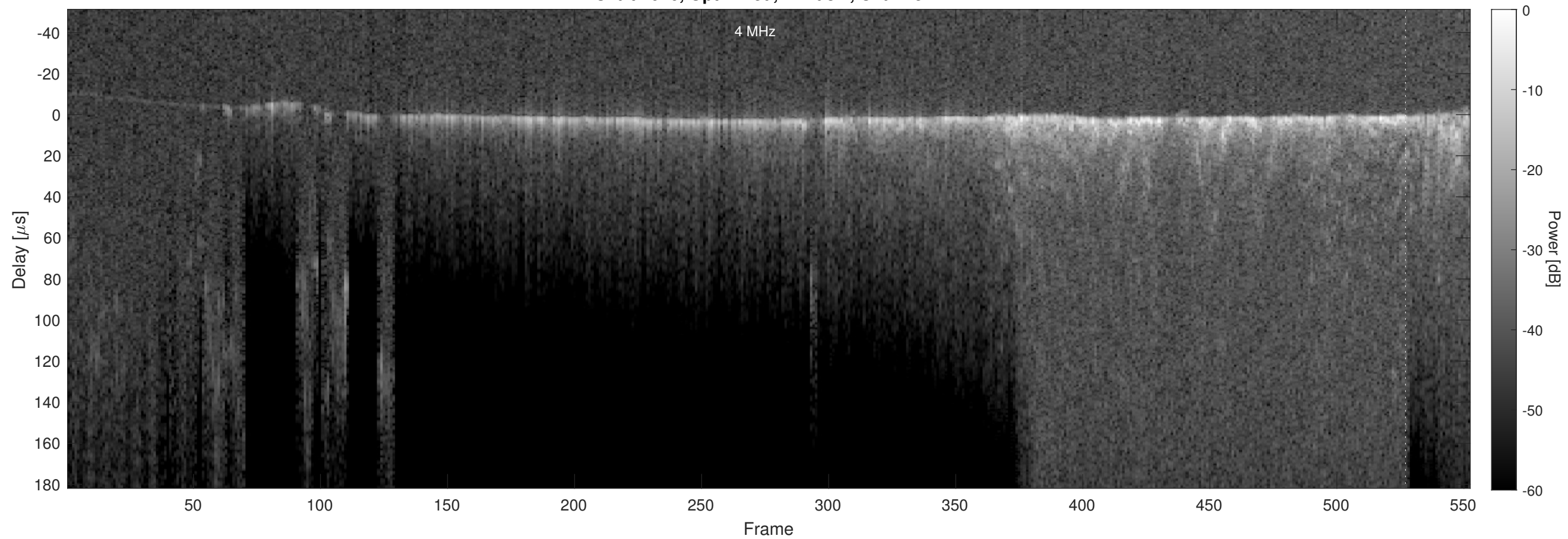
Orbit 2026, Optimized, Window, Channel 2
