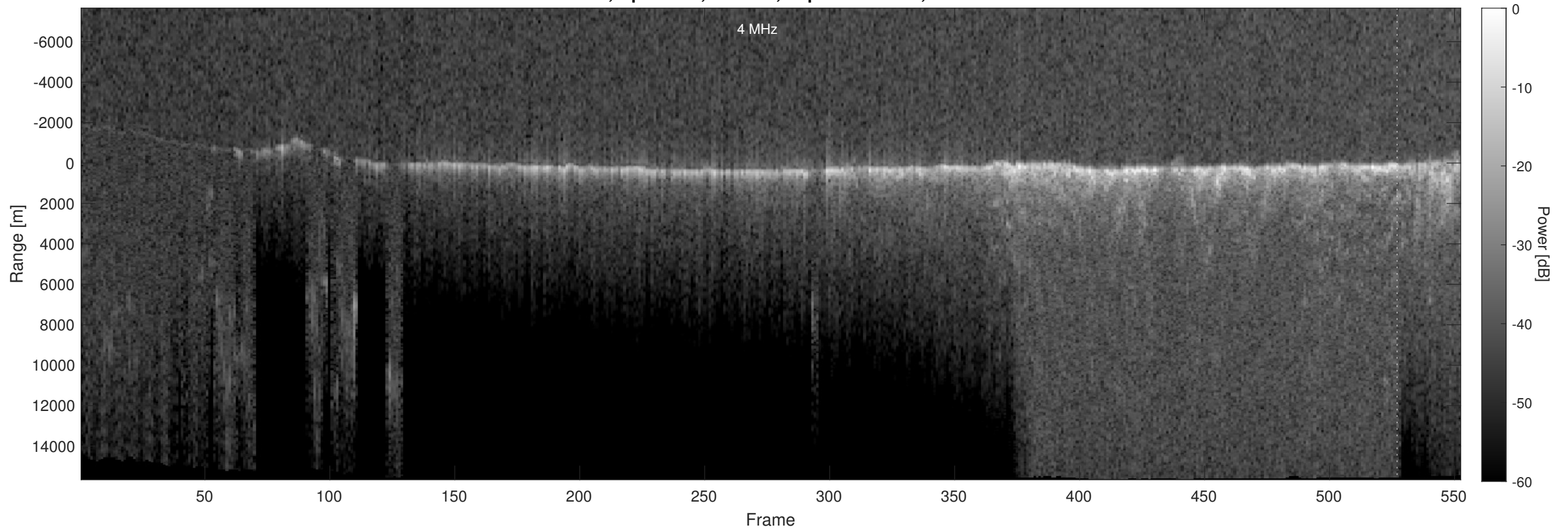
Orbit 2026, Optimized, Window, Depth-Corrected, Channel 2
