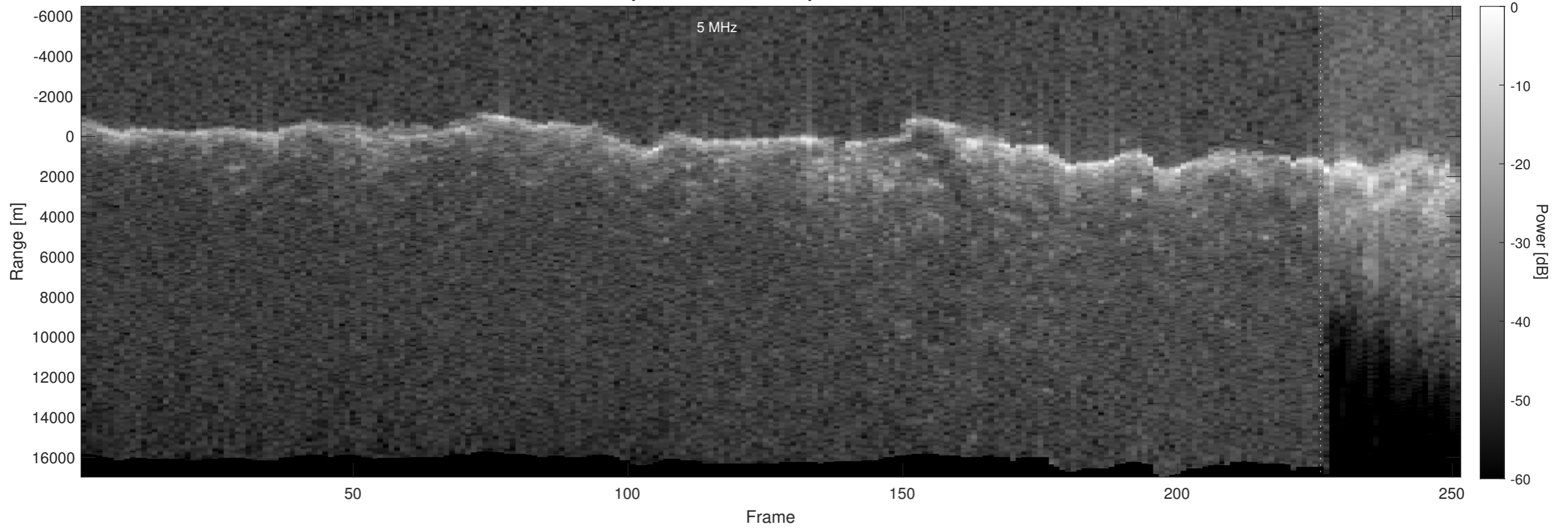
Orbit 2027, Optimized, Window, Depth-Corrected, Channel 2
