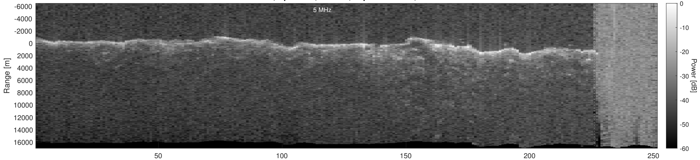
Orbit 2027, Optimized, Window, Depth-Corrected, Channel 2
