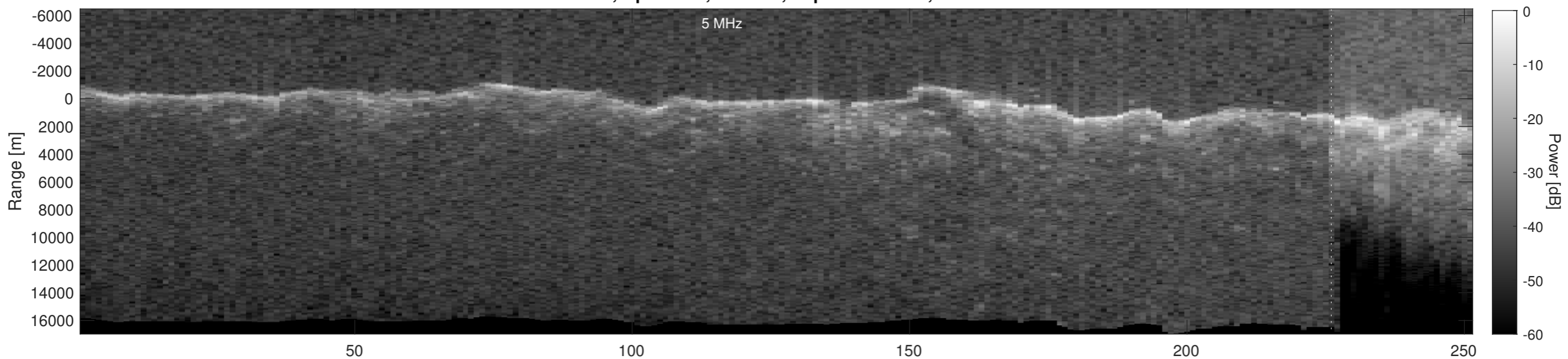
Orbit 2027, Depth-Corrected Cluttergram
