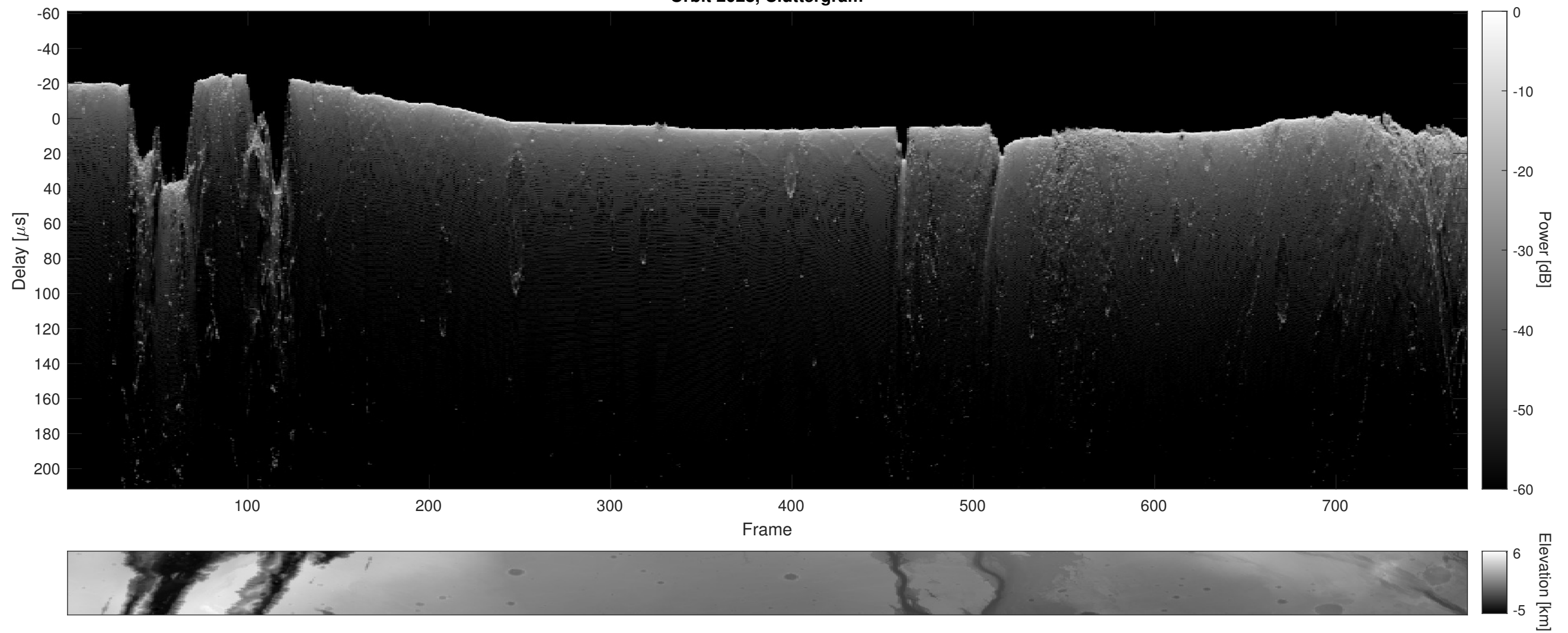
Orbit 2028, Cluttergram
