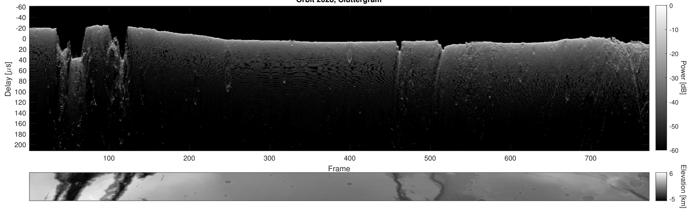
Orbit 2028, Cluttergram
