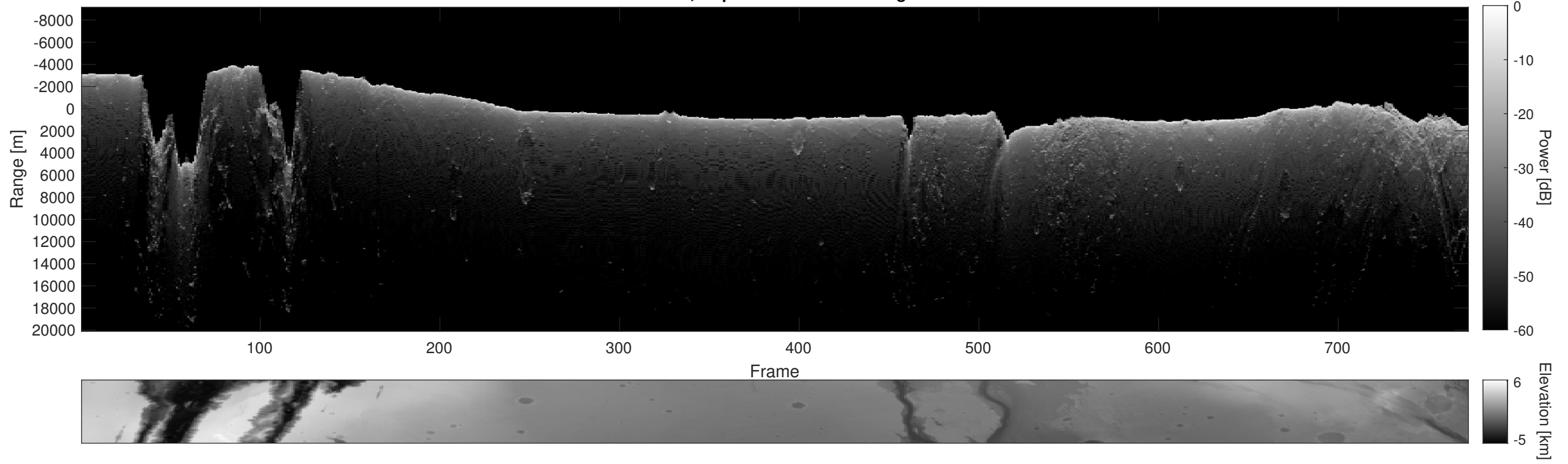
Orbit 2028, Depth-Corrected Cluttergram
