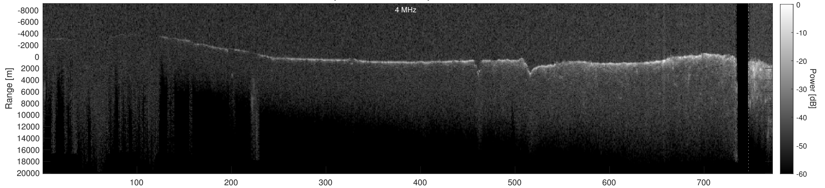
Orbit 2028, Depth-Corrected Cluttergram
