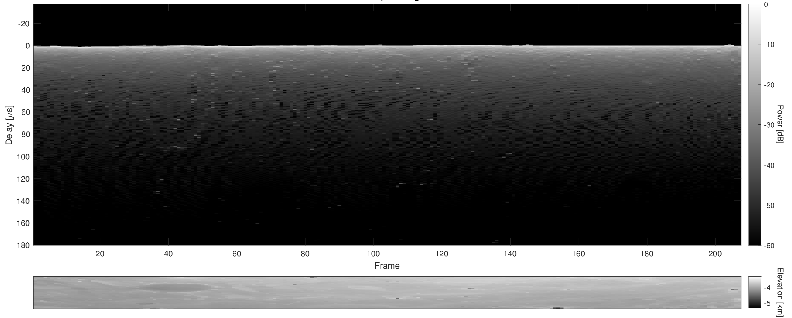
Orbit 2035, Cluttergram
