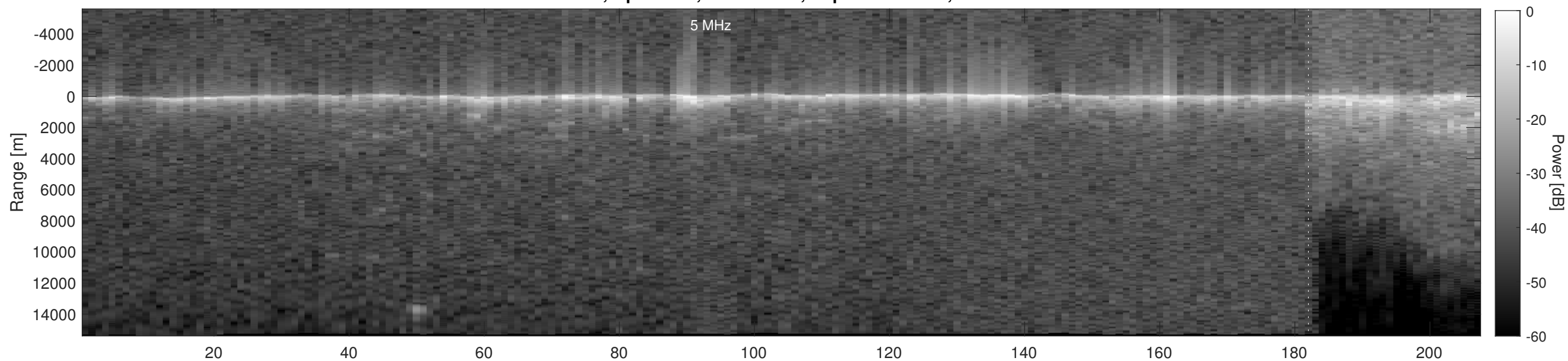
Orbit 2035, Depth-Corrected Cluttergram
