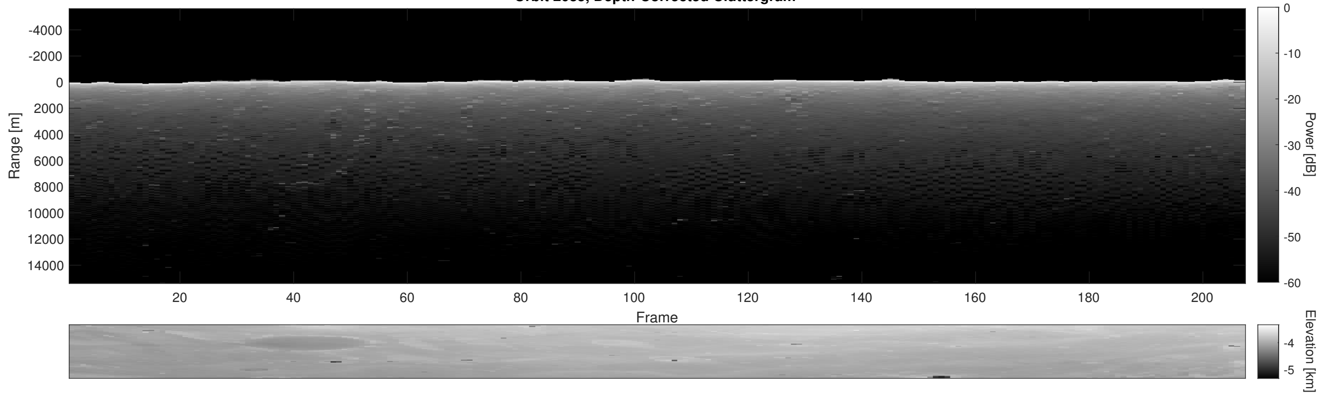
Orbit 2035, Depth-Corrected Cluttergram
