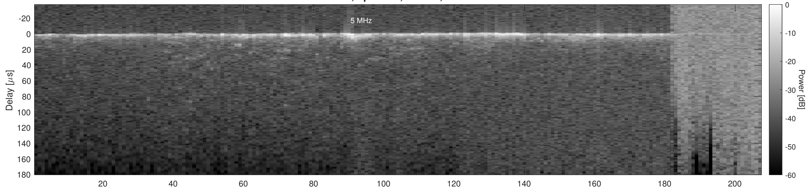
Orbit 2035, Optimized, Window, Channel 2
