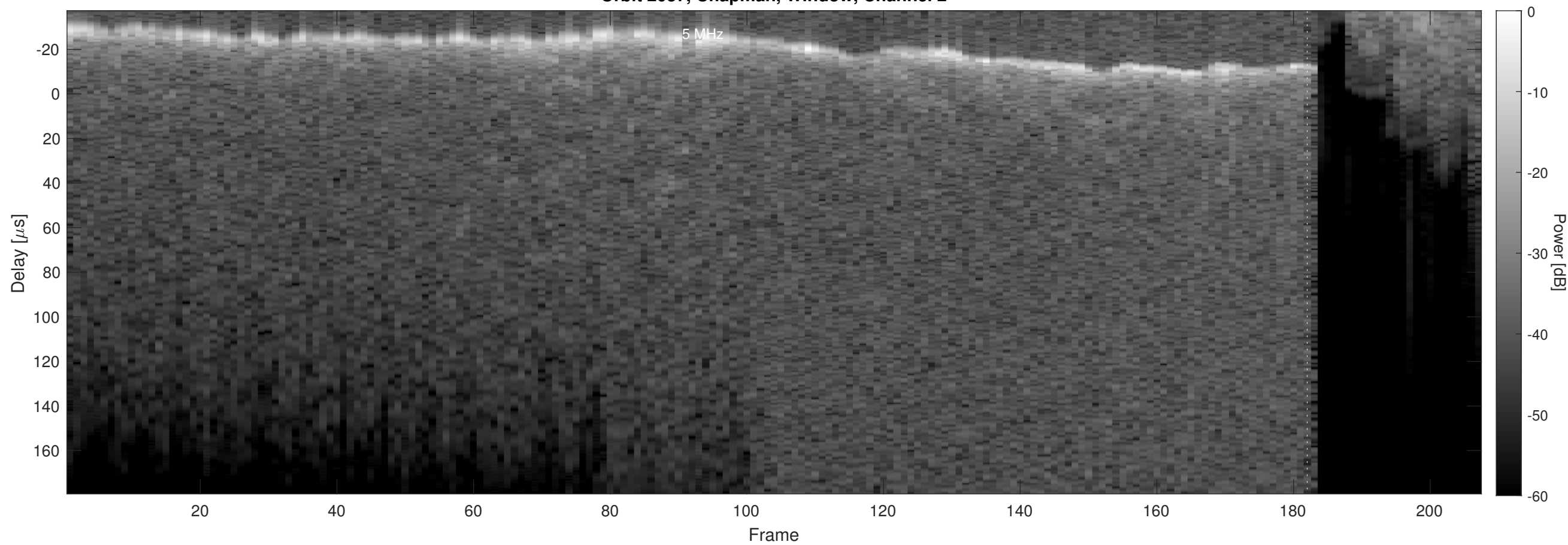
Orbit 2037, Chapman, Window, Channel 2
