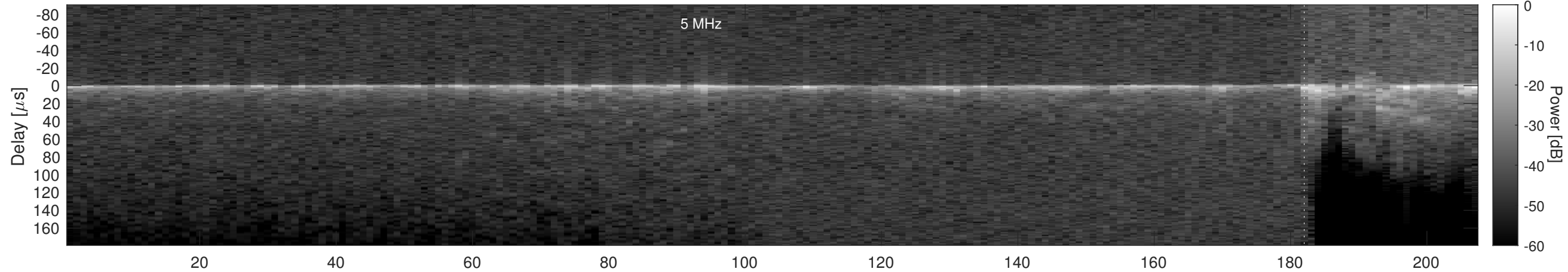
Orbit 2037, Cluttergram
