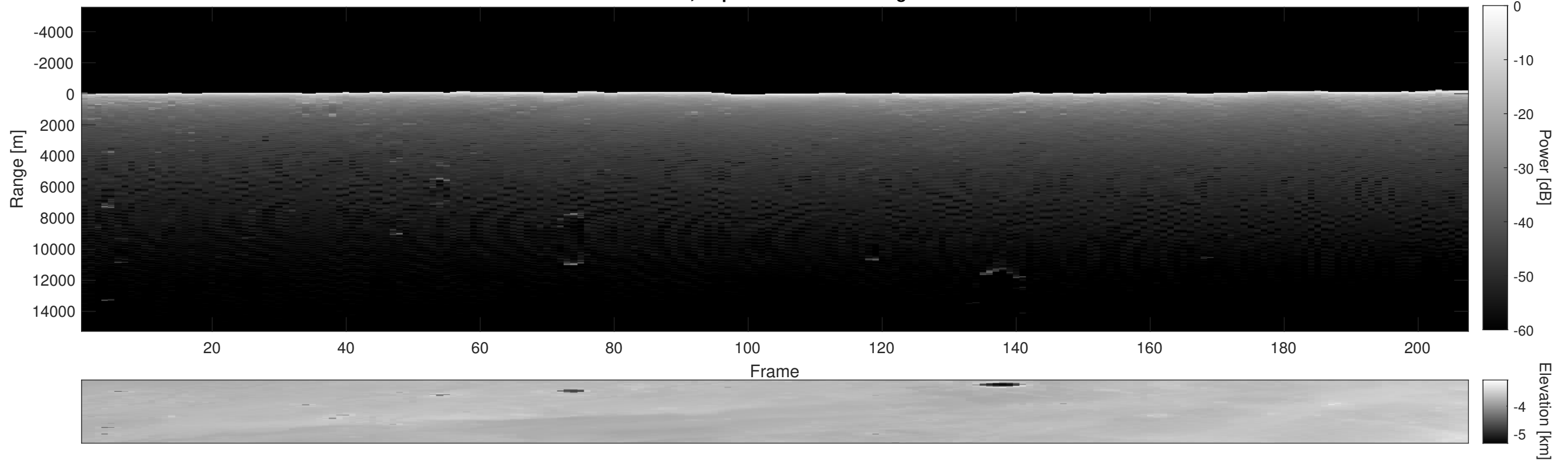
Orbit 2037, Depth-Corrected Cluttergram
