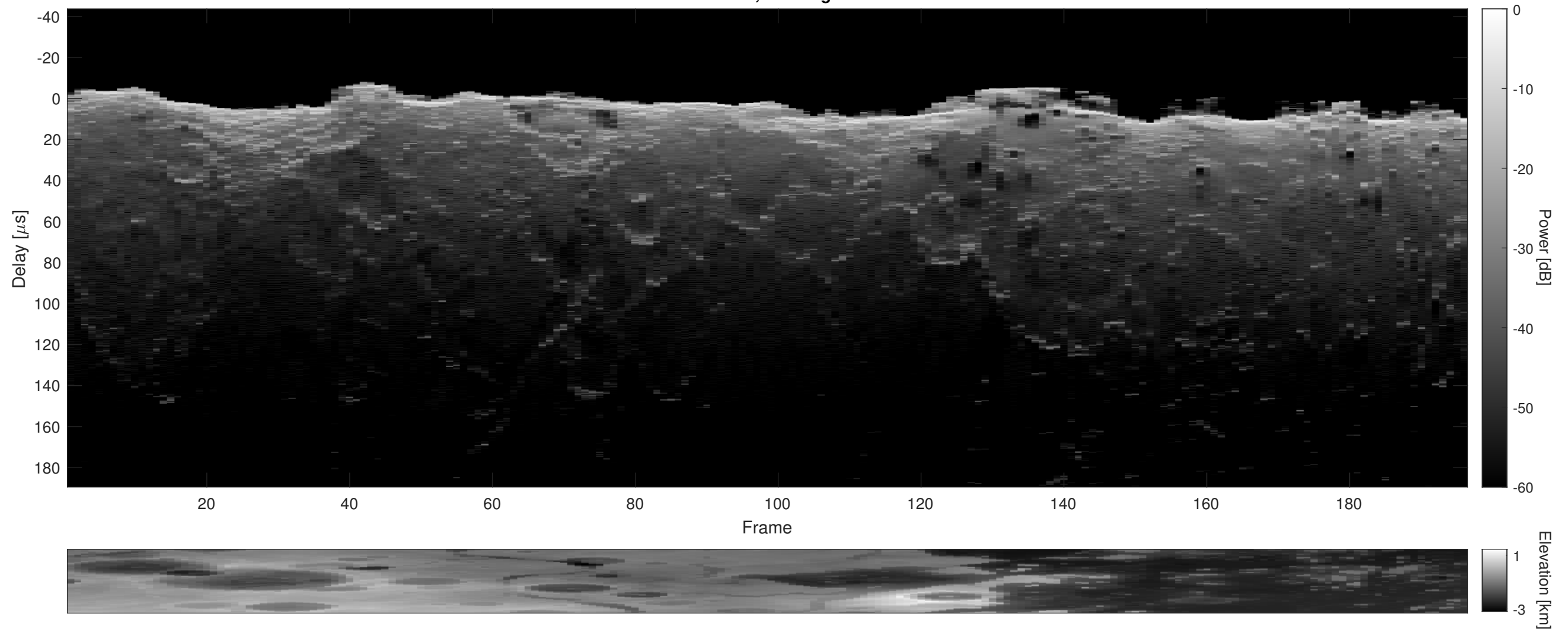
Orbit 2038, Cluttergram
