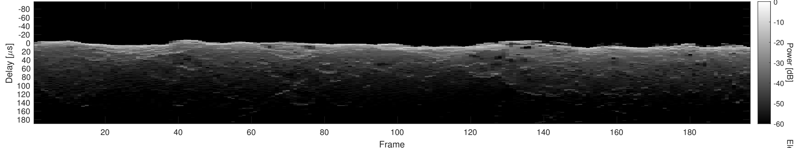
Orbit 2038, Cluttergram
