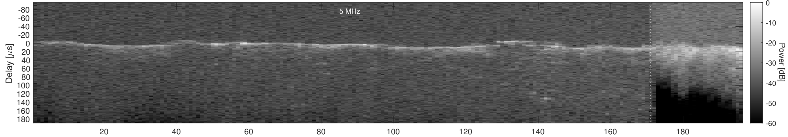
Orbit 2038, Cluttergram
