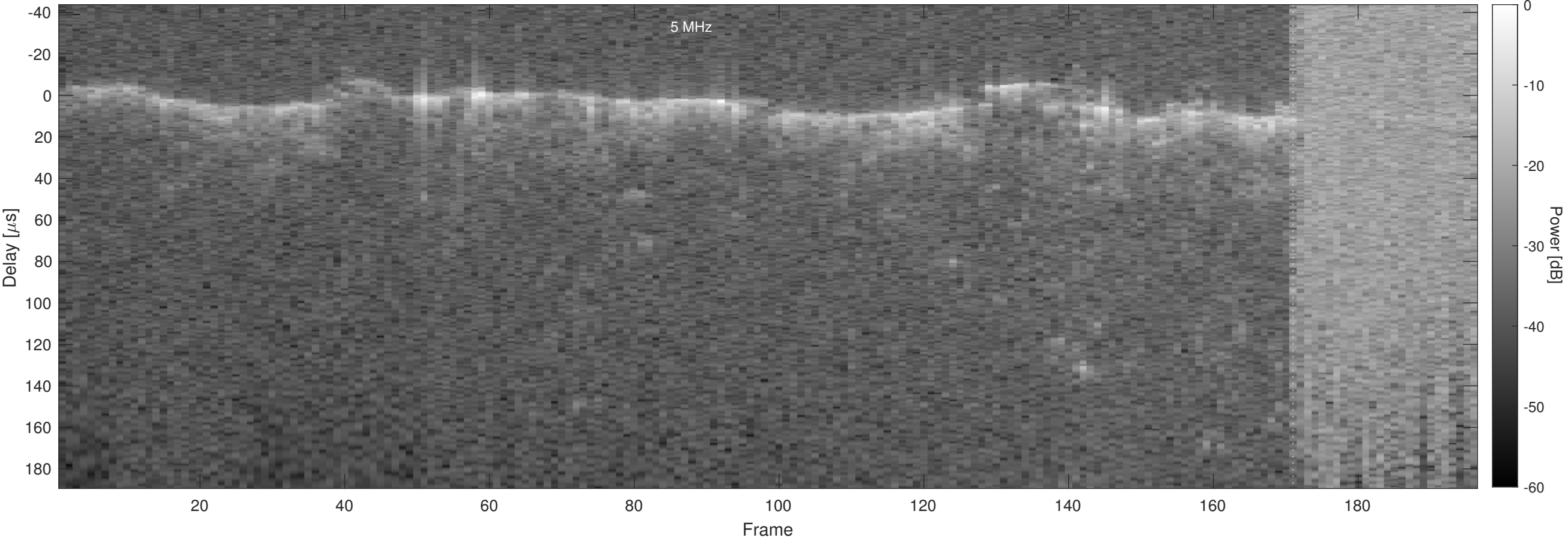
Orbit 2038, Optimized, No Window, Channel 2
