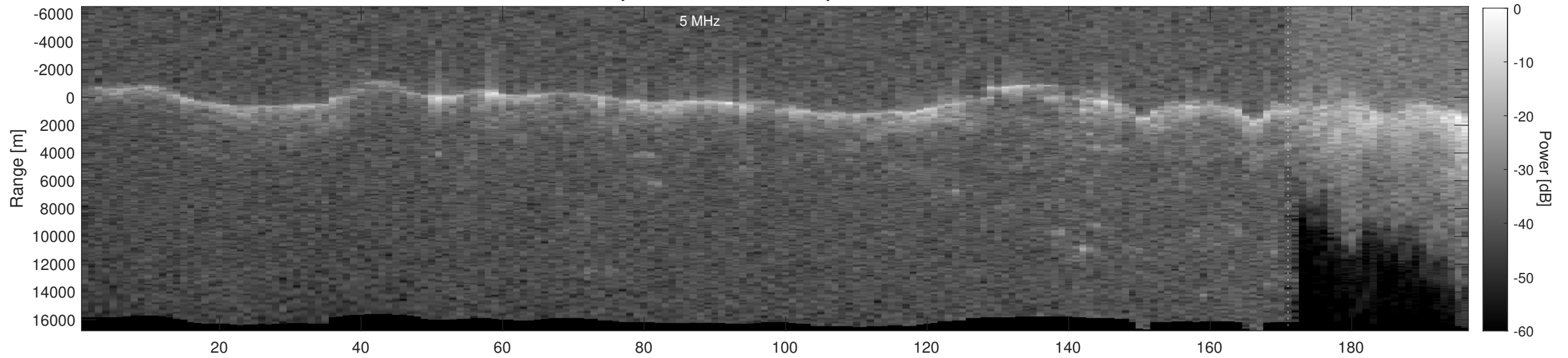
Orbit 2038, Depth-Corrected Cluttergram
