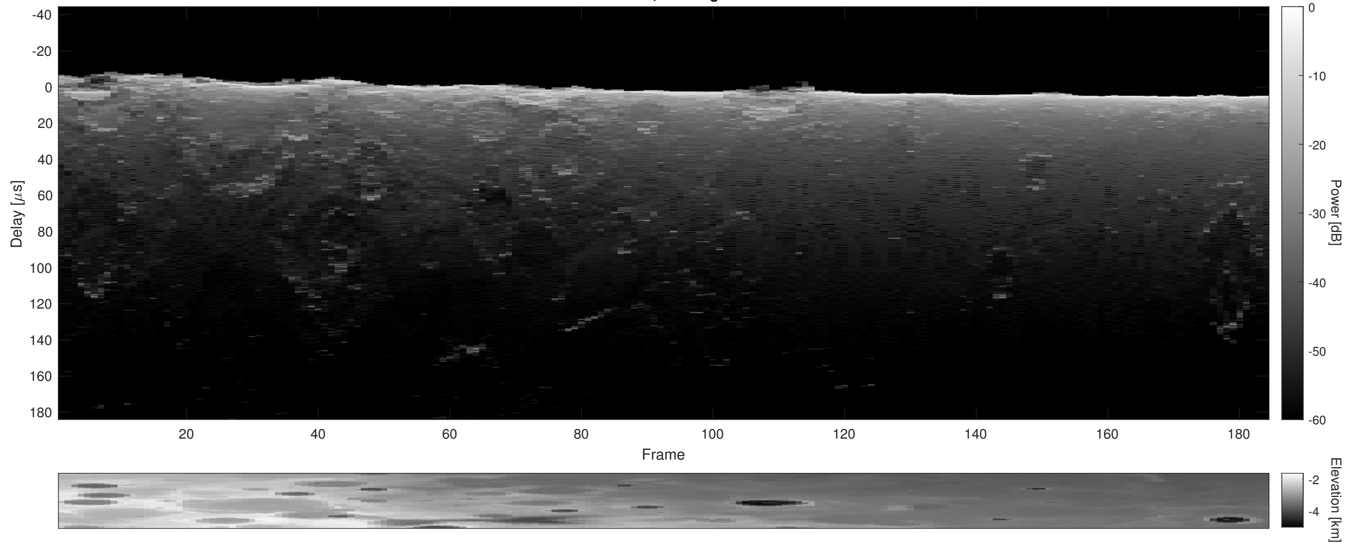
Orbit 2042, Cluttergram
