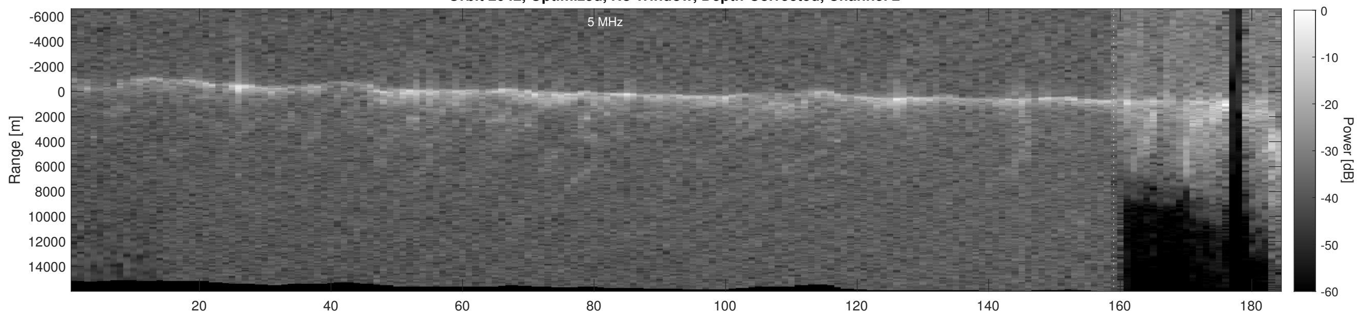
Orbit 2042, Depth-Corrected Cluttergram
