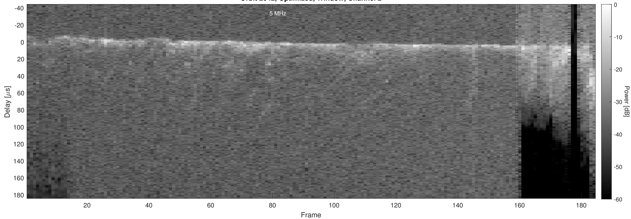
Orbit 2042, Optimized, Window, Channel 2
