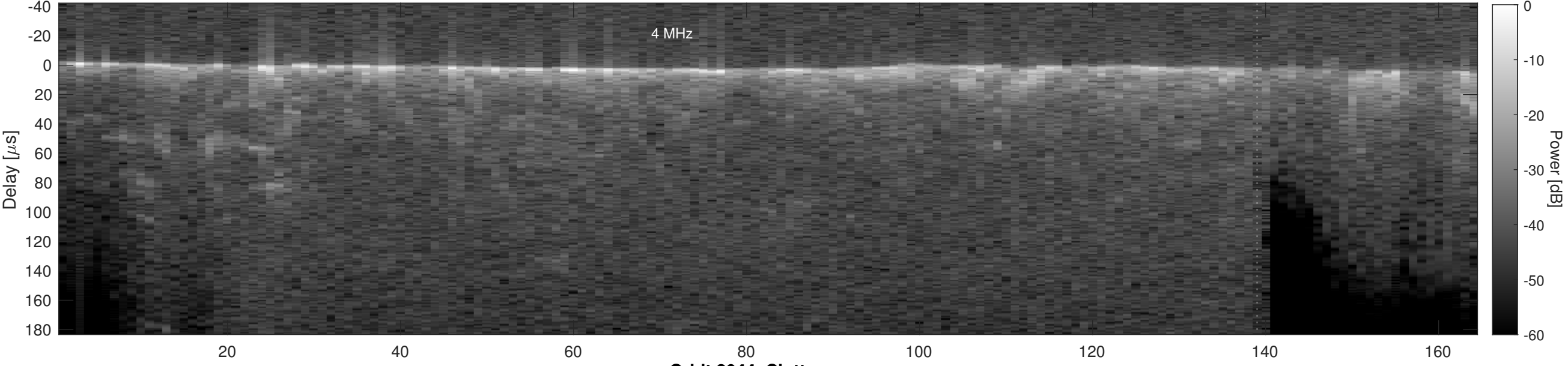
Orbit 2044, Cluttergram
