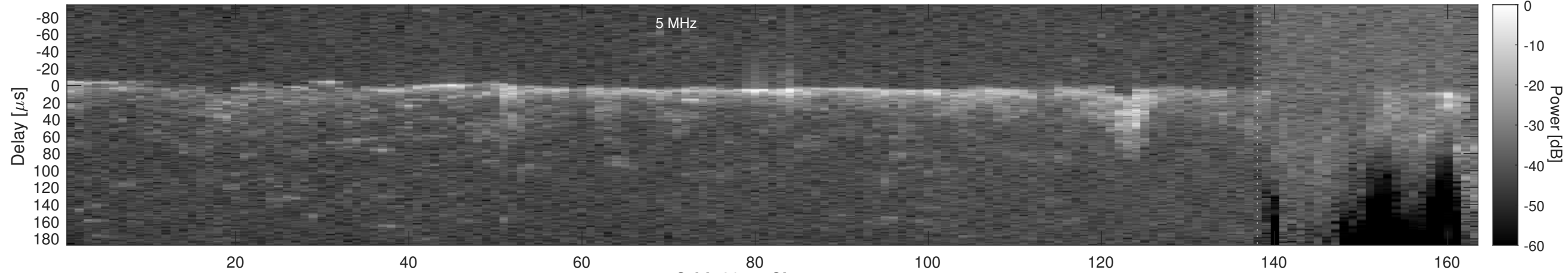
Orbit 2045, Cluttergram
