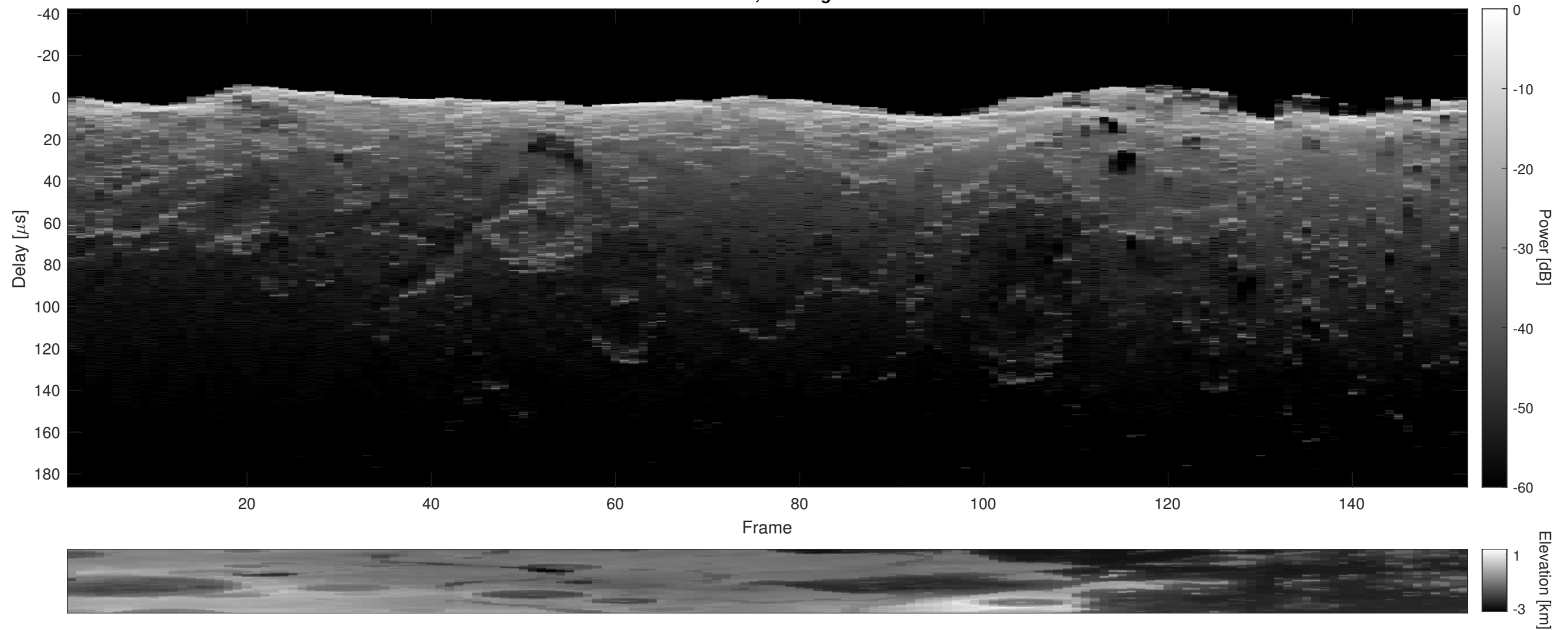
Orbit 2049, Cluttergram
