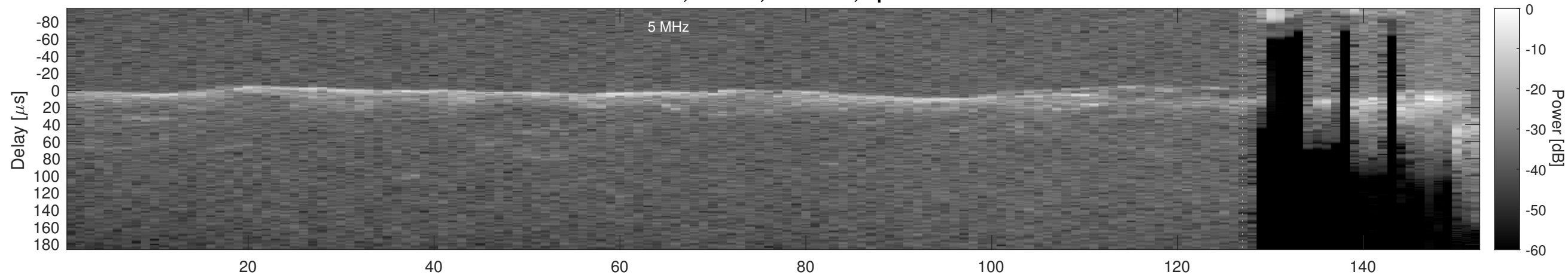
Orbit 2049, Cluttergram
