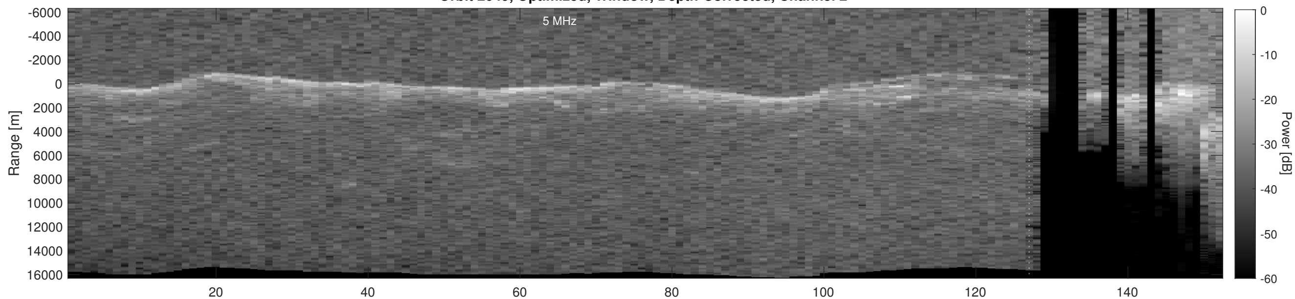
Orbit 2049, Depth-Corrected Cluttergram
