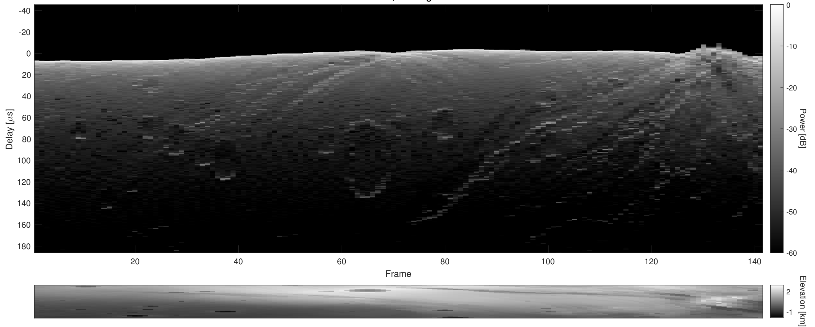
Orbit 2050, Cluttergram
