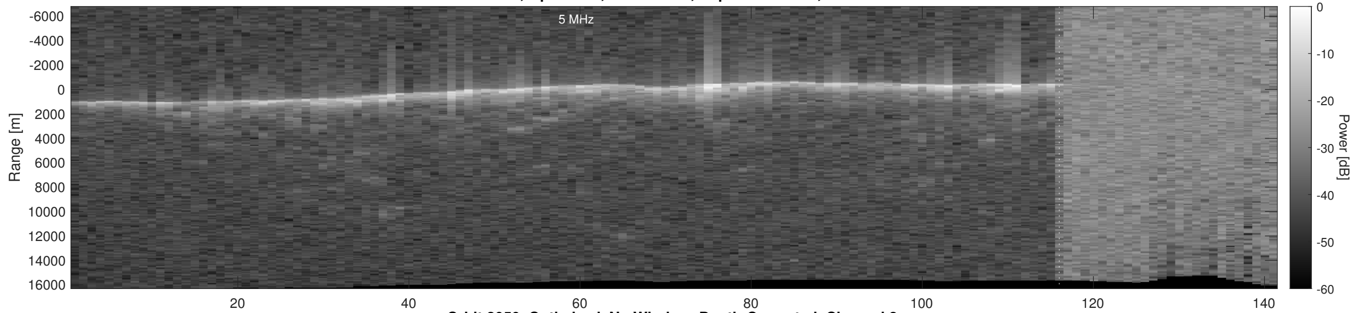
Orbit 2050, Optimized, No Window, Depth-Corrected, Channel 2
