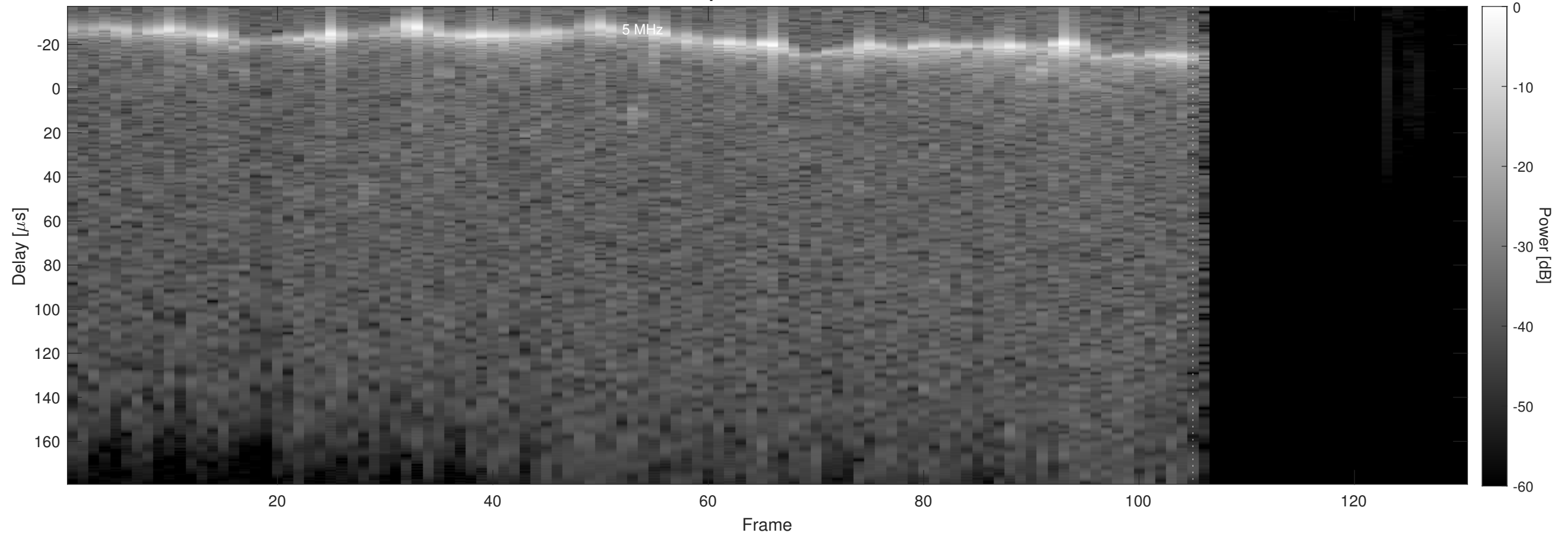
Orbit 2052, Chapman, No Window, Channel 2
