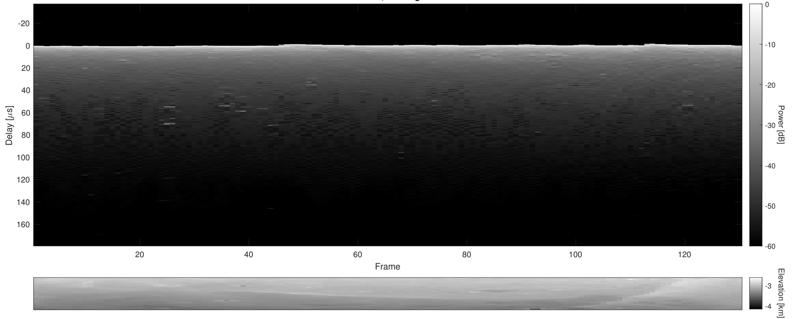
Orbit 2052, Cluttergram
