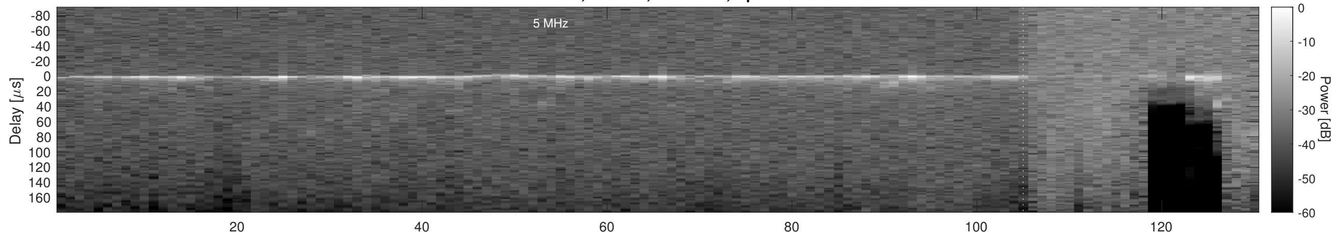
Orbit 2052, Cluttergram
