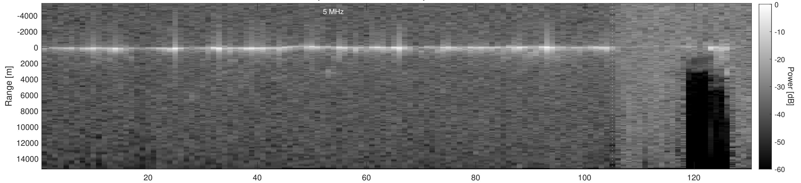
Orbit 2052, Depth-Corrected Cluttergram
