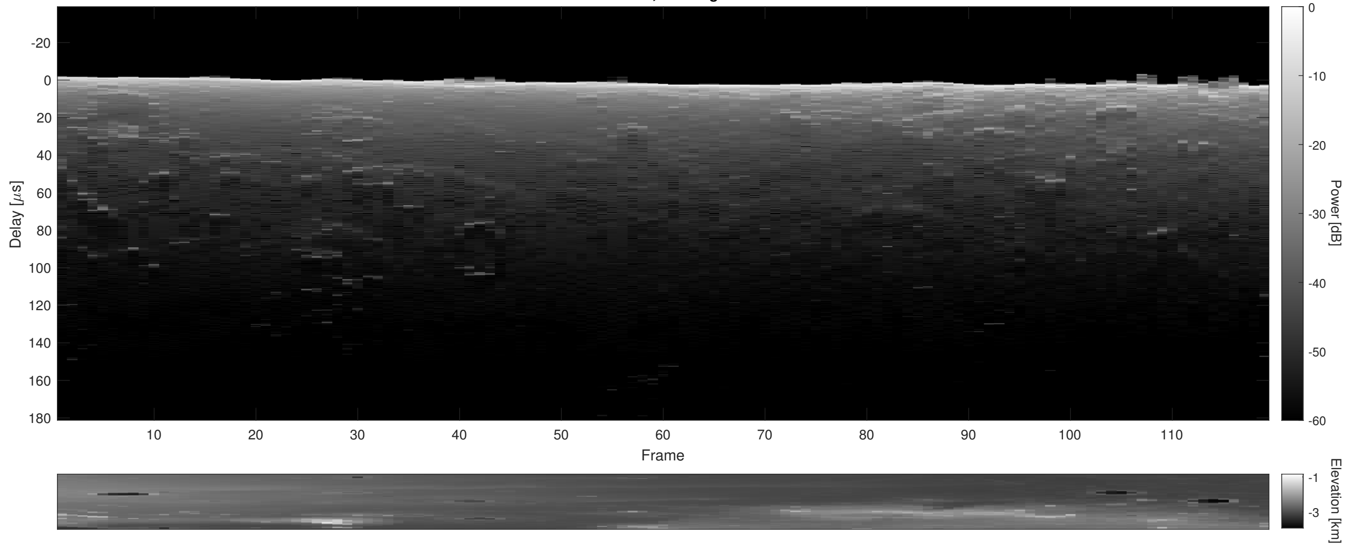
Orbit 2055, Cluttergram
