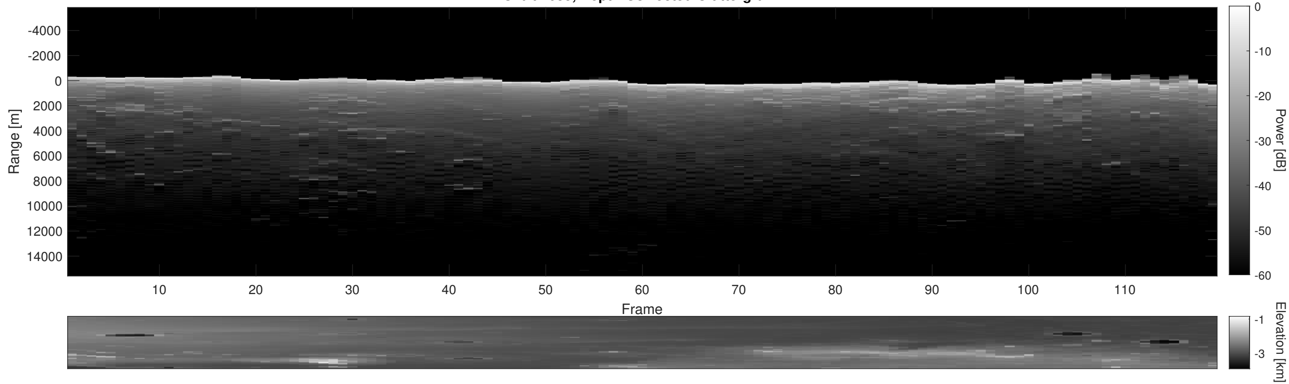
Orbit 2055, Depth-Corrected Cluttergram
