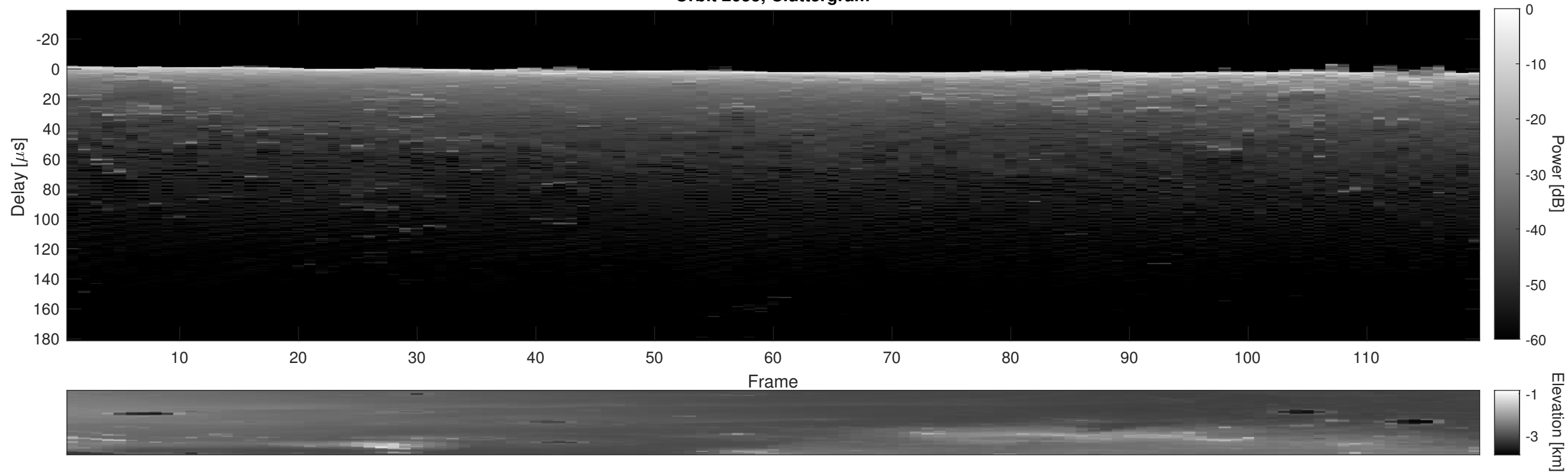
Orbit 2055, Cluttergram
