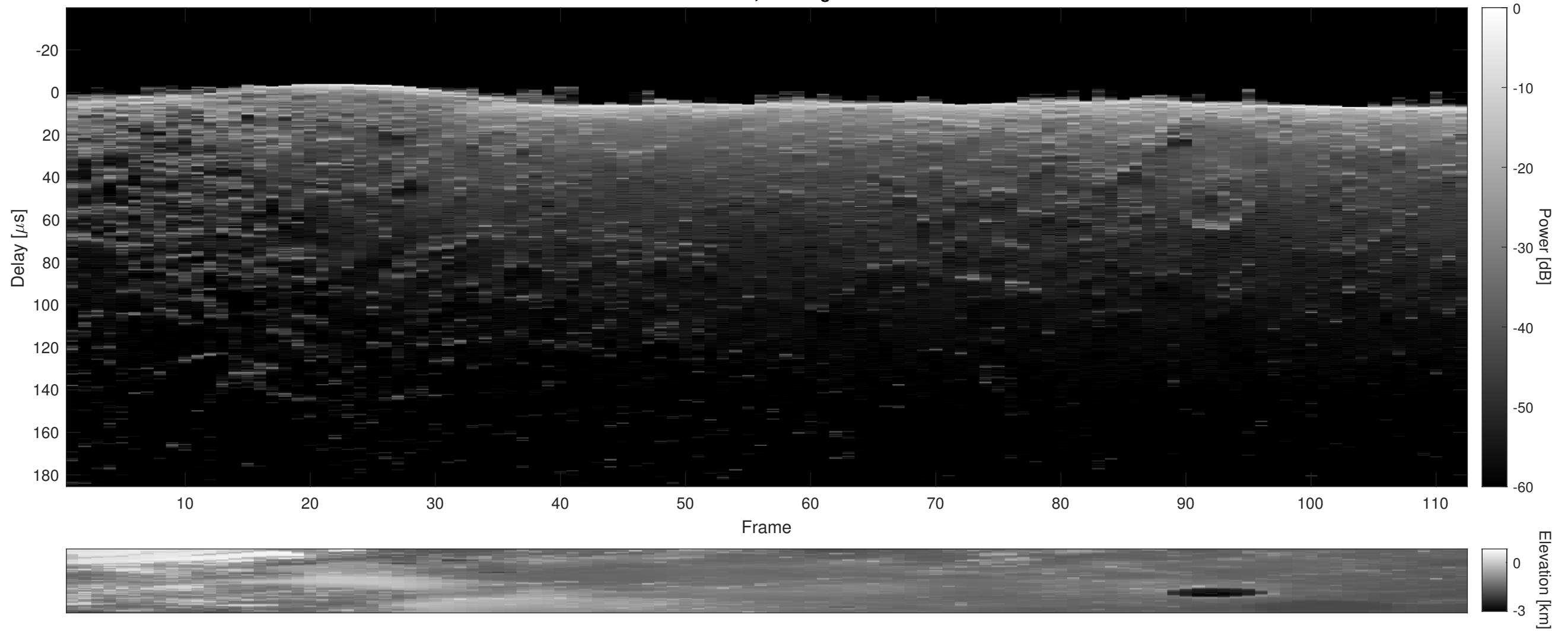
Orbit 2056, Cluttergram
